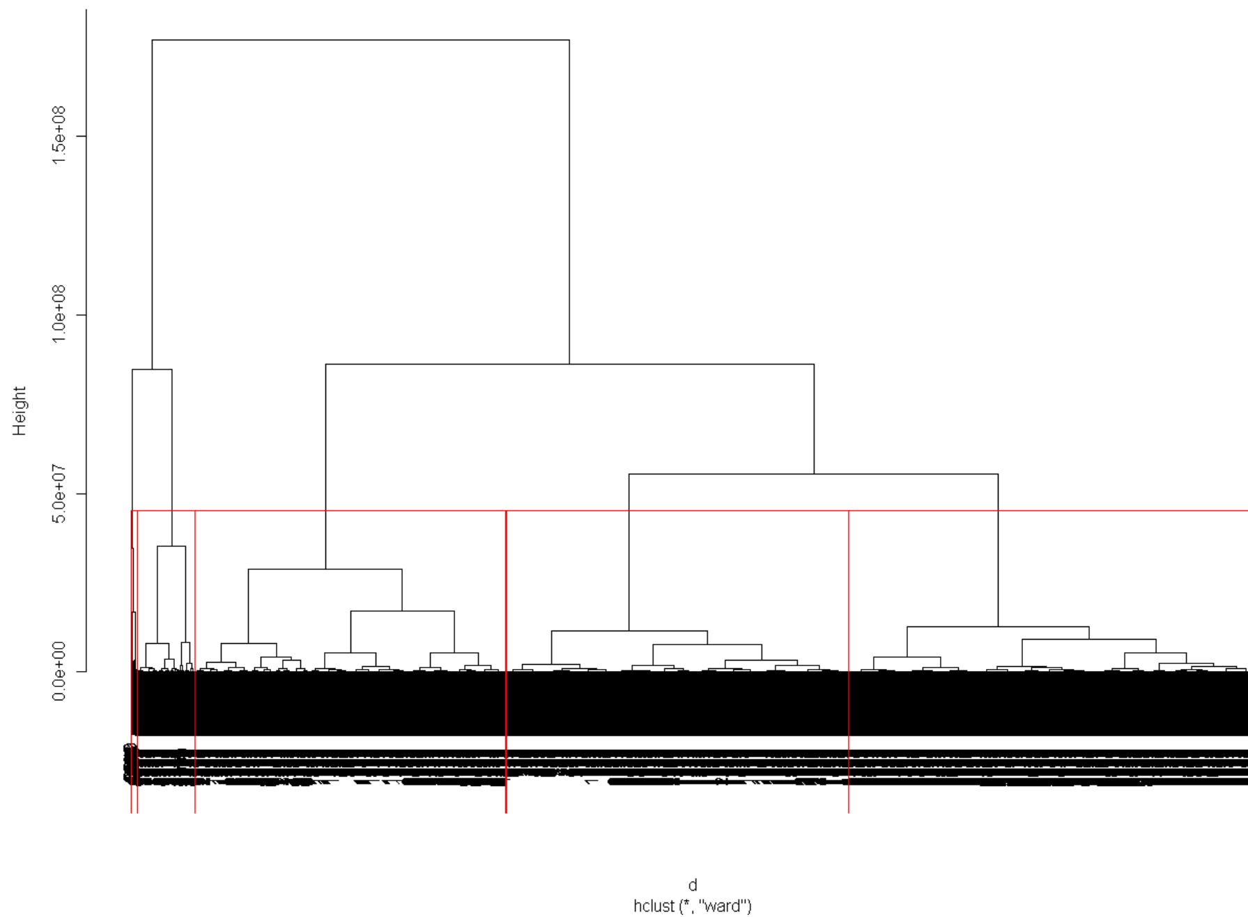
Cluster Dendrogram
